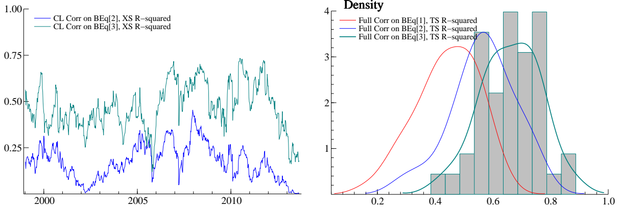
Figure 2: R-squared statistics
