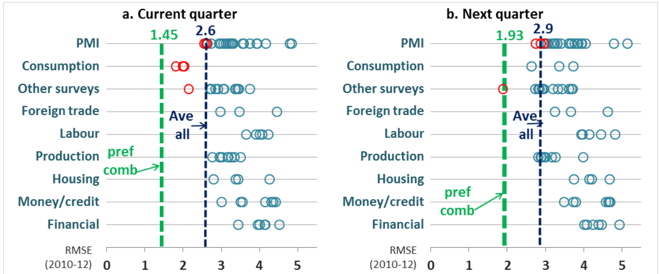
Figure 9. Japan: RMSE
