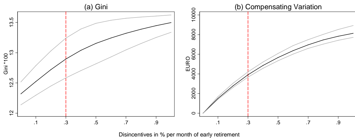
Figure 5: Gini and CVs by disincentive level
