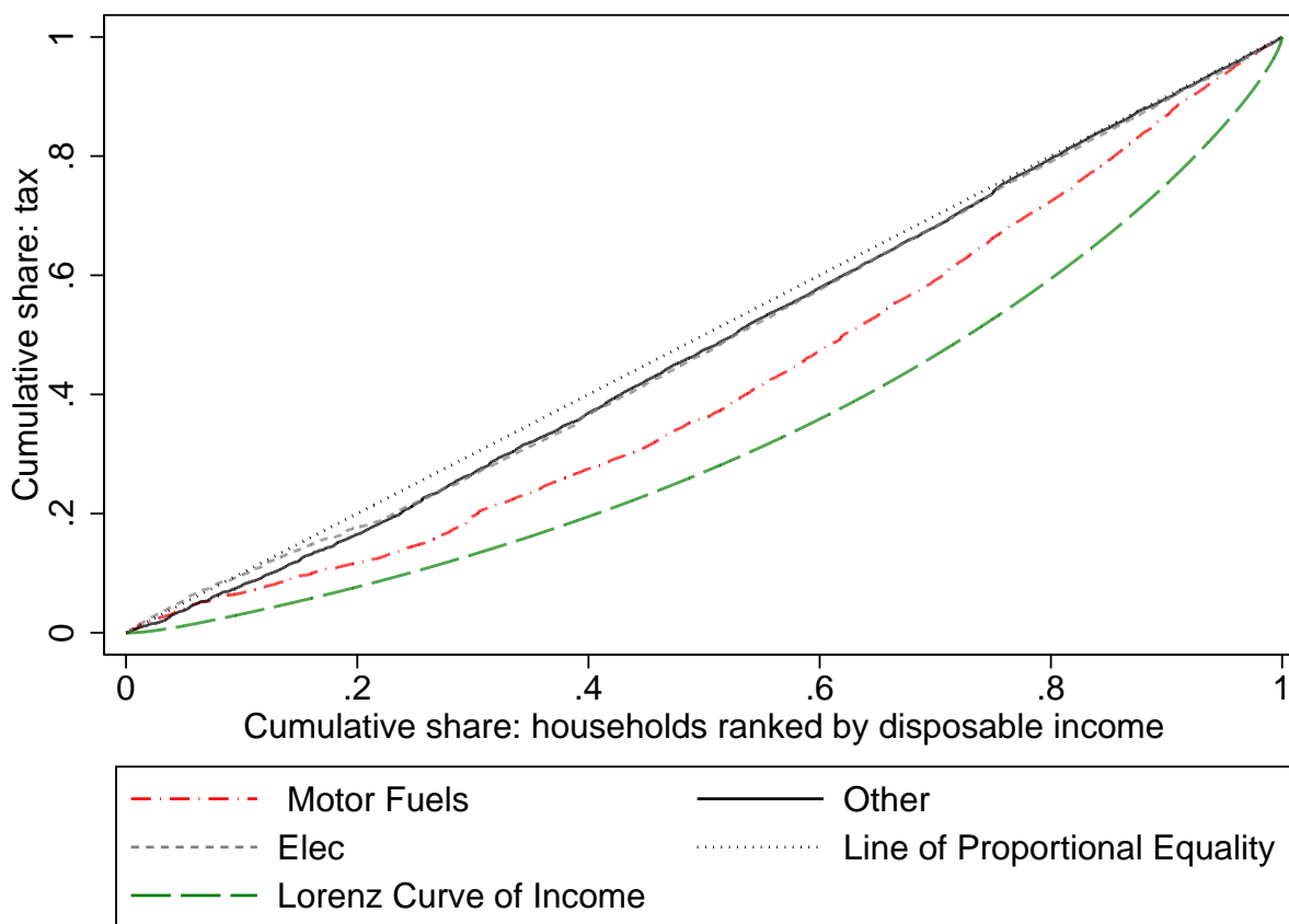
Figure 1: Lorenz curve and concentration curves
