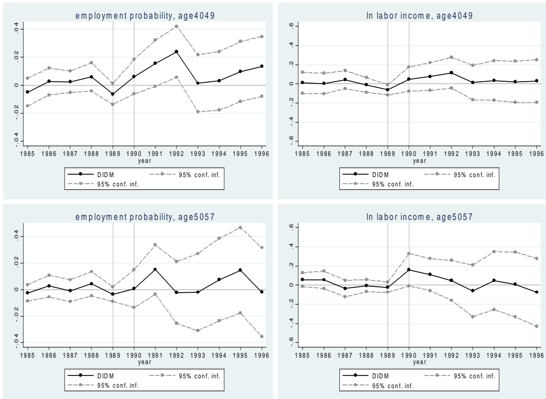
Note: The figures show the difference-in-differences matching estimates, \hat{\alpha}_{DIDM} (see equation (3)): The point estimate for each year shows the difference in mean outcome between the treatment group and the matched control group that year, above the difference in mean outcome between the groups for 1985-1989. The sample used for the estimations for age 2229 contains 1369 treatment individuals and 2282 potential control individuals. The corresponding figures for age 3039 (4049) [5057] are 2526 (2859) [1152] and 3362 (3800) [1857] respectively.
