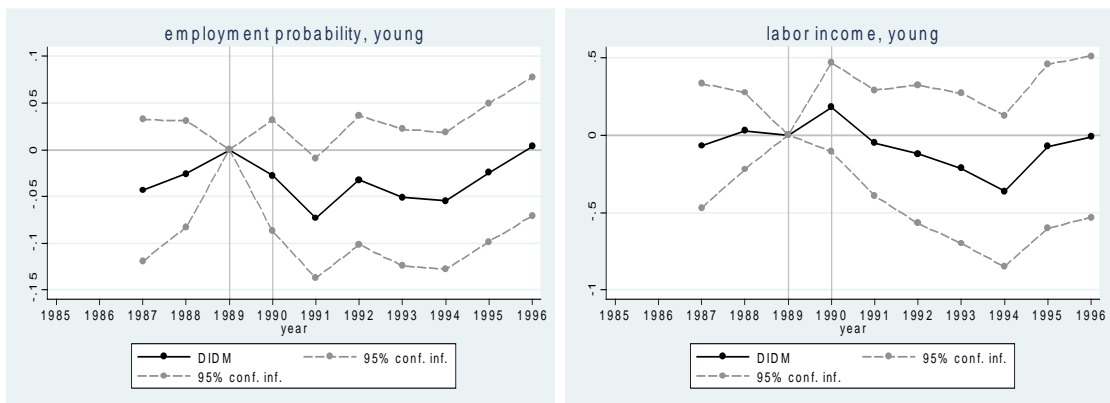
Note: The figures show the difference-in-differences matching estimates, \hat{\alpha}_{DIDM} (see equation (3)): The point estimate for each year shows the difference in mean outcome between the treatment group and the matched control group that year, above the difference in mean outcome between the groups for 1989. The sample used for the estimations contains 647 treatment individuals and 897 potential control individuals. Young is defined as being 19-21 years old in 1989. For young people, the labor income and employment history variables in the set of X used in the algorithm to choose the propensity score only include values for 1988 and 1989.
