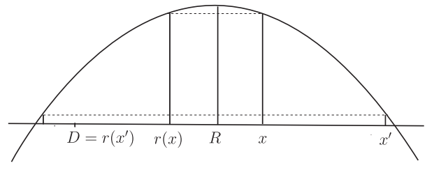
Figure 5: r(\cdot)
