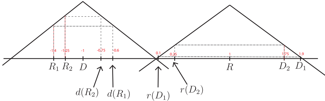
Figure 1: Example 1
