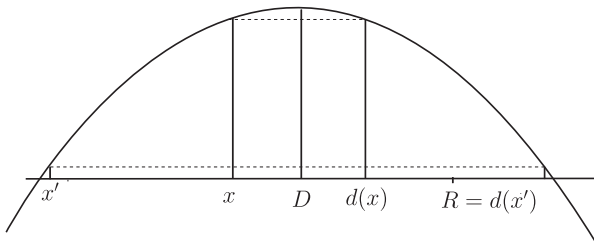
Figure 4: d(\cdot)
