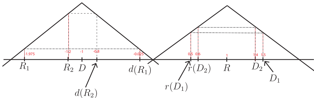
Figure 3: Examples 3 and 4
