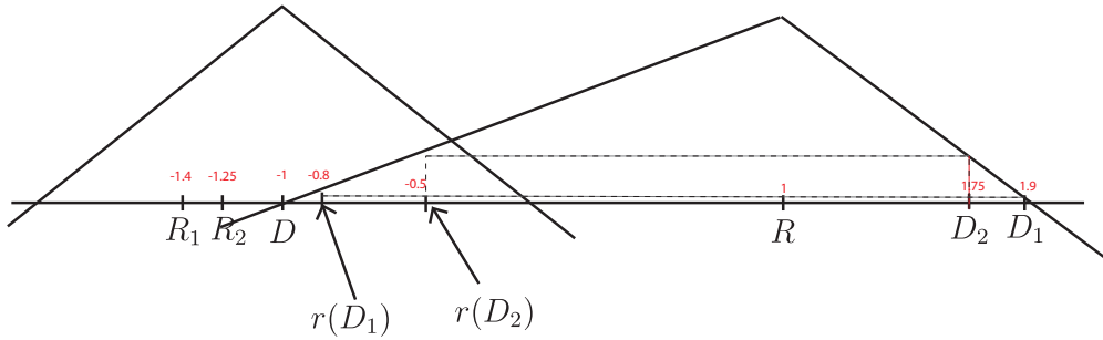
Figure 2: Example 2
