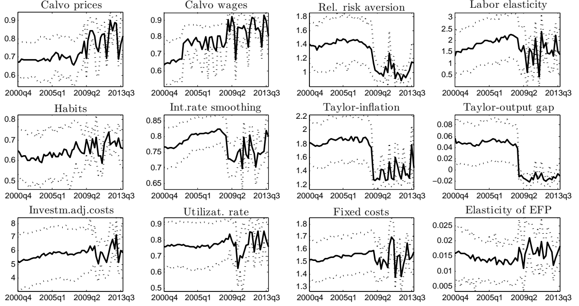
Figure 7: Evolution of the parameters of the BGG model, where the observable financial variable is credit spread. Solid lines represent the posterior mean, while dotted lines 5th and 95th posterior percentiles. Estimates are computed based on the recursive estimation sample starting from 1984Q1-2000Q4 and ending in 2013Q4.
