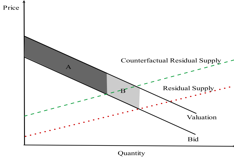
Figure 9: Statistical effect
