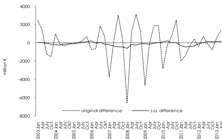
Figure 4: Original and seasonally adjusted difference between direct and indirect SA of gross fixed capital formation
