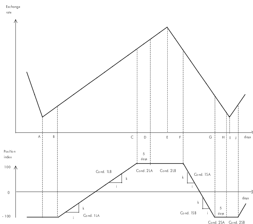
Figure 7: Exchange trends and aggregate positions of technical models
