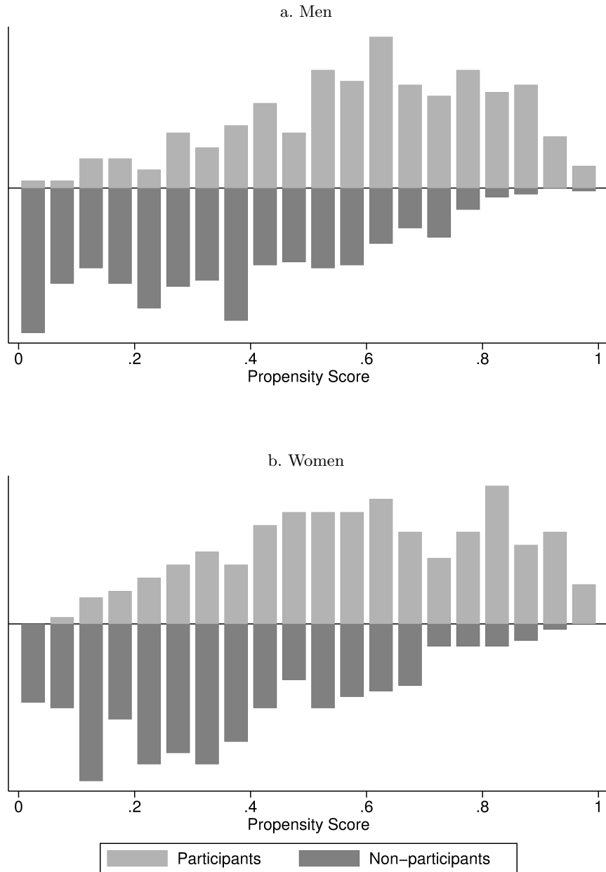
Figure 1: Propensity score distributions
