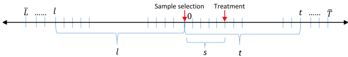
Figure 2: Graphical Representation of the Notation
