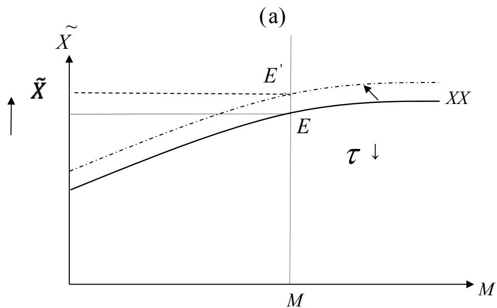
Figure A1. Determination of aggregate intermediate good usage under exogenous M
