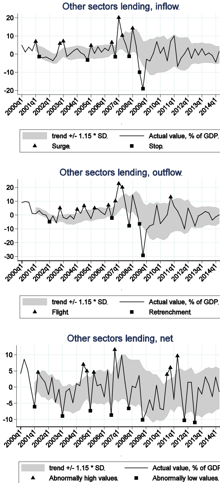
Figure B11: Other Sectors Lending Flows (% of GDP)
