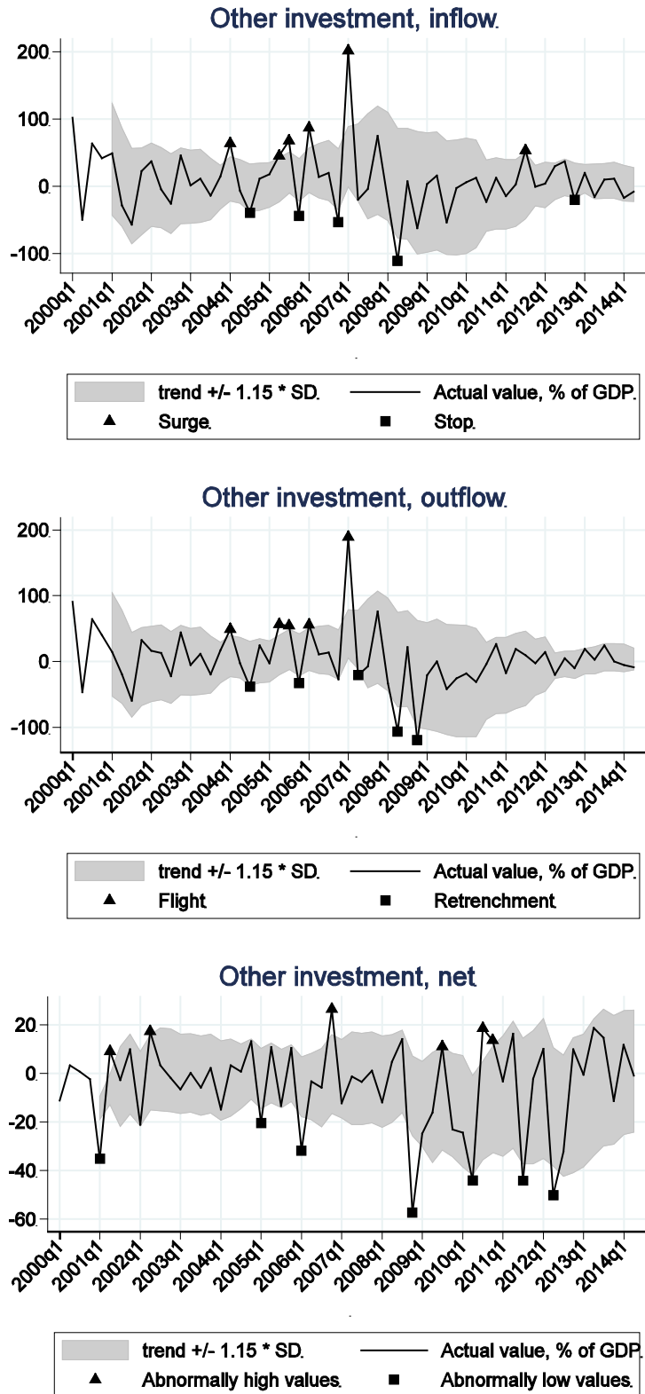
Figure B9: Other Investment Flows (% of GDP)
