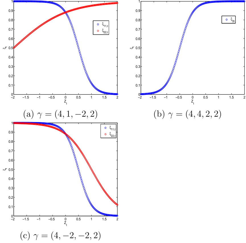
Figure 1: Some examples: Nonlinear effect of the covariate on the state persistence
