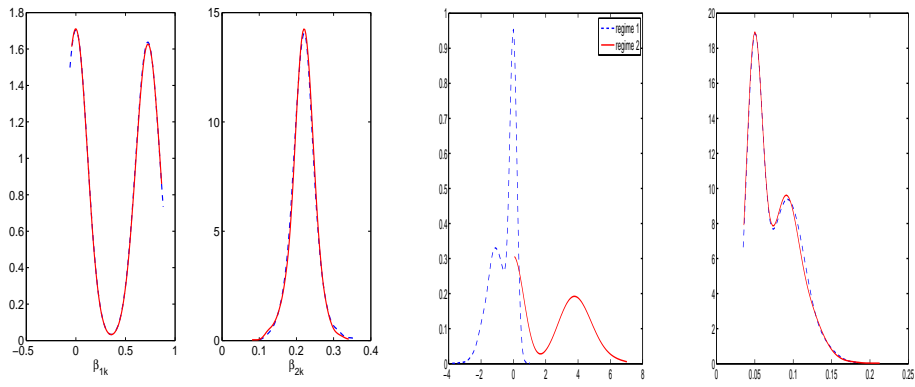
Figure 2: Random permutation with dRUM auxiliary sampling for the transition distribution. Marginal distribution of selected parameters.
