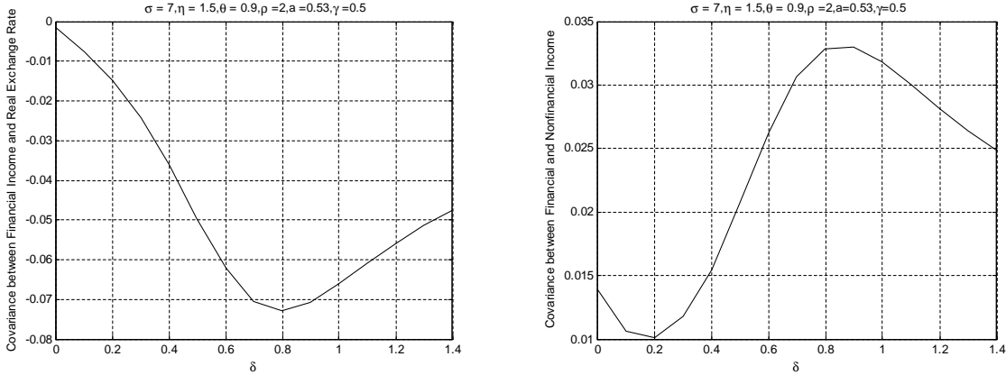
Figure 4: Covariance Relationships
