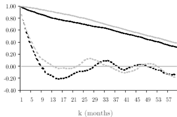
(b) Autocorrelation Coefficients: DPR
