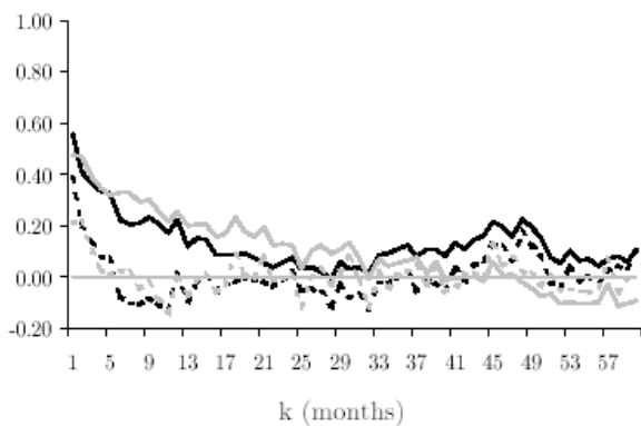
(f) Autocorrelation Coefficients: VOLA
