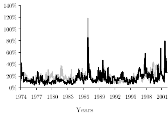
(e) Realized Stock Market Volatility
