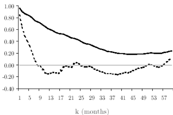
(h) Autocorrelation Coefficients: DEF
