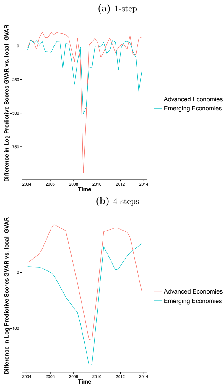
Figure 4: Performance of regional GVAR models
