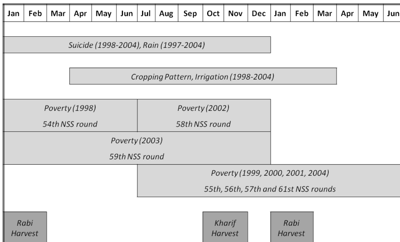
Figure 4: Data Matching
