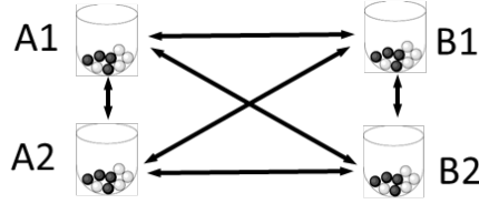
Figure 5: Data structure
