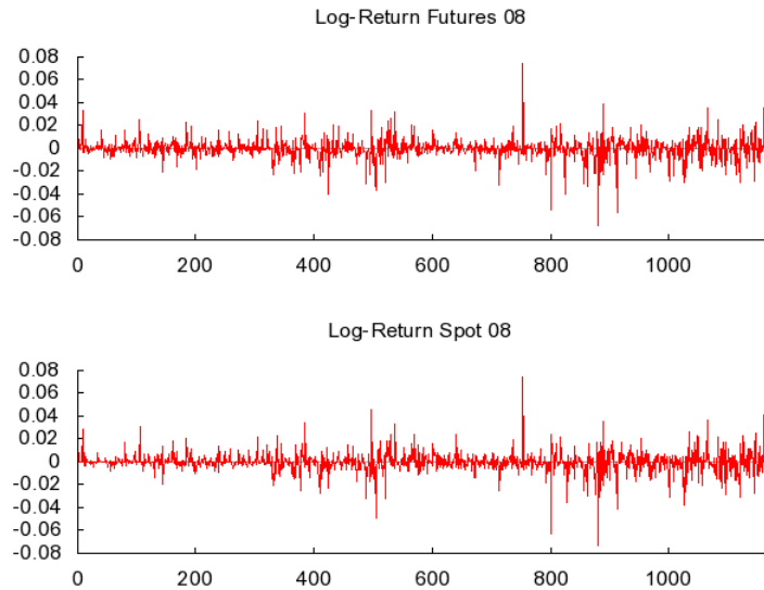
Figure 2: Log>Returns in the spot and futures market based on the contract with maturity in December 2008 and frequency h = 60 minutes.
