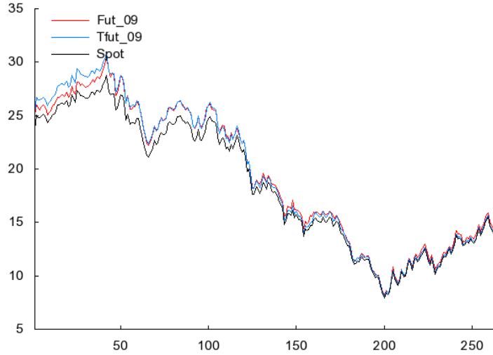
Figure 1: Cost-of-Carry Relationship: Contract with maturity in Dec 2009
