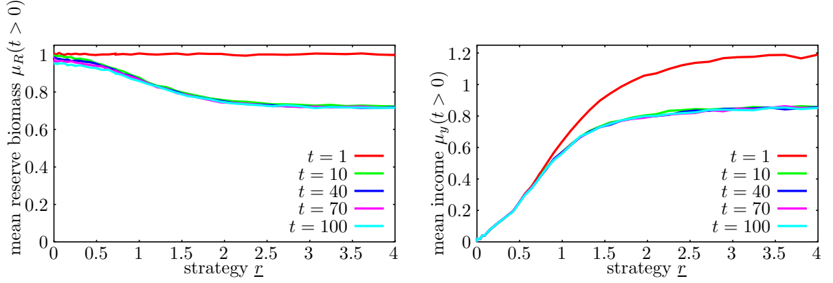
Figure 10: Parameter values are as in Figure 6, except for w_G = 4 .
