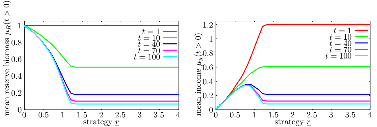
Figure 11: Parameter values are as in Figure 6, except for \sigma_r = 0.05 .
