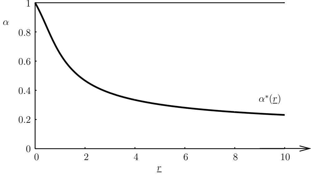
Figure 3: The set of feasible strategies is given by the whole area \alpha \in [0, 1] , r \in [0, \infty) . The set of efficient strategies for parameters \mu_r = 1.2 and \sigma_r = 0.7 is the curve.
