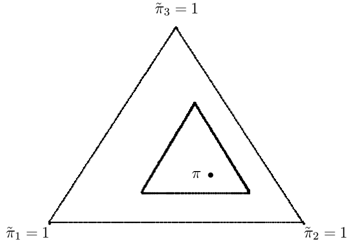
Figure 3: Multiple priors
