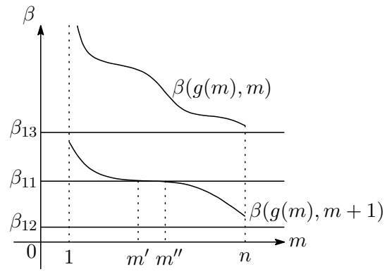
Figure 3: Sufficiency
