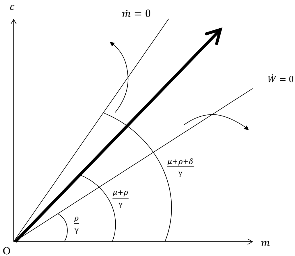
Figure 6: Persistent growth ( \beta = 0 )
