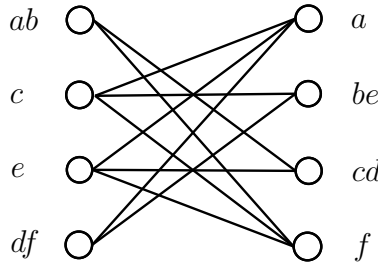
Figure 7: G(S_1, S_2)
