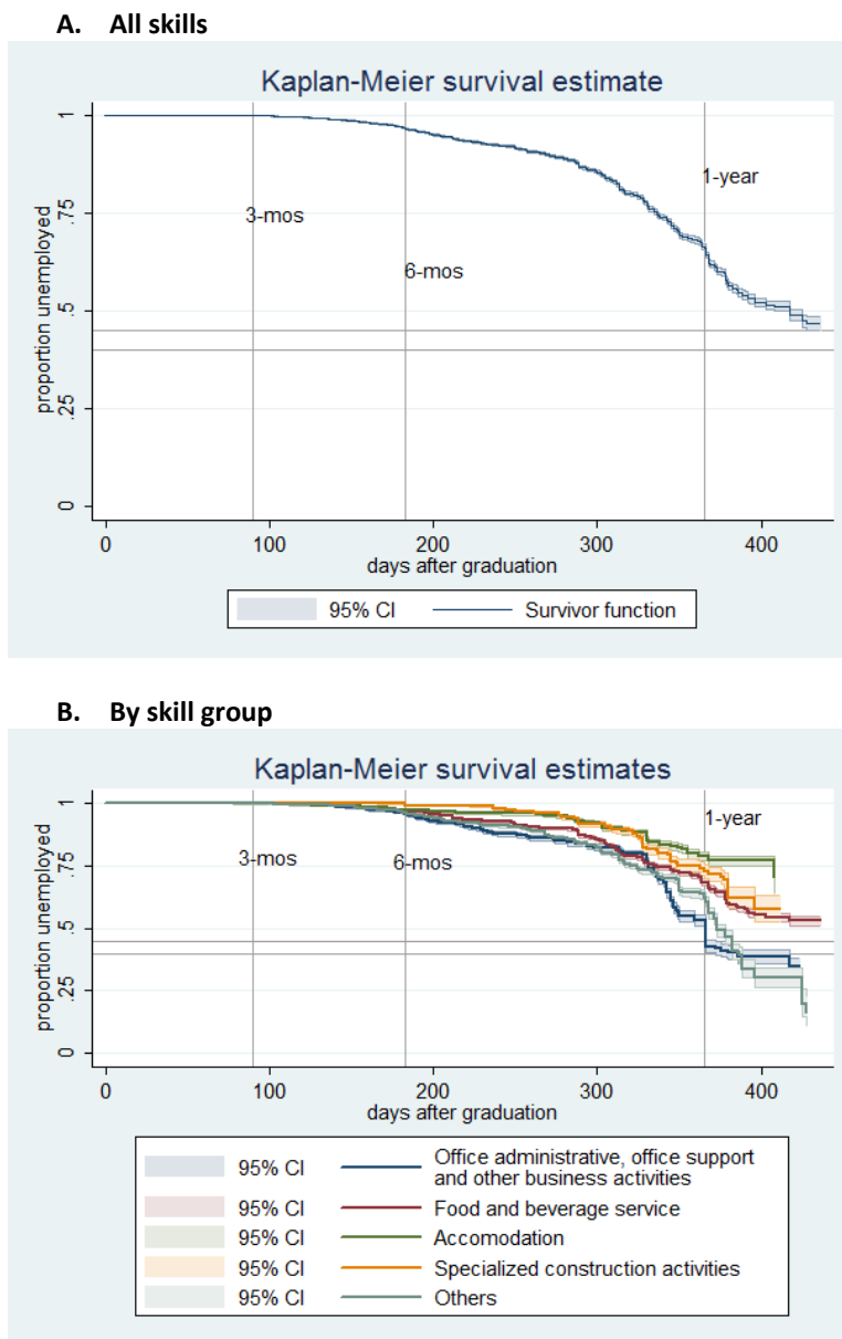
Figure 3. Unemployment Duration
