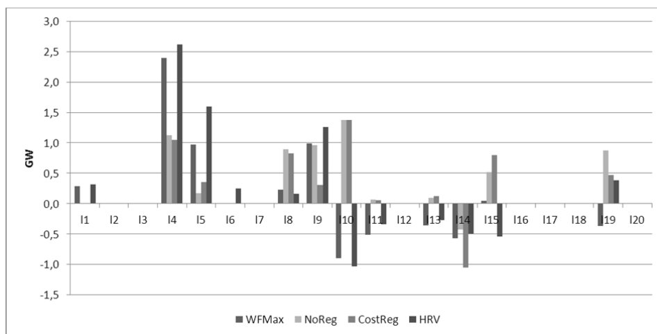
Figure 10: Line extension differences between baseline and the case with increased wind capacity (final period)
