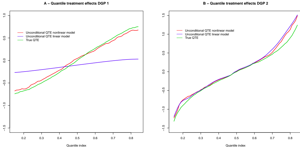
Figure 4: Based on N = 10'000 . The figure displays unconditional QTE estimates based on the semiparametric plug-in approach, unconditional QTE estimates obtained from a linear model, and the true unconditional QTE.
