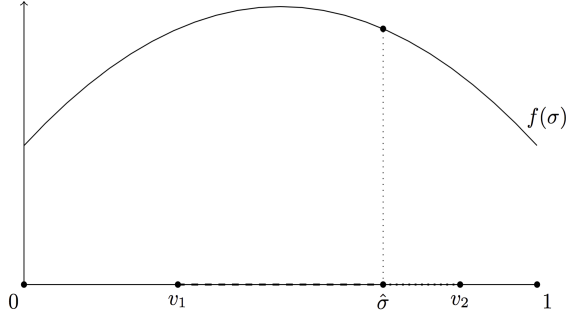
Figure 1: Illustration of an outcome given v_1 and v_2 where the ideal approach is \hat{\sigma} .
