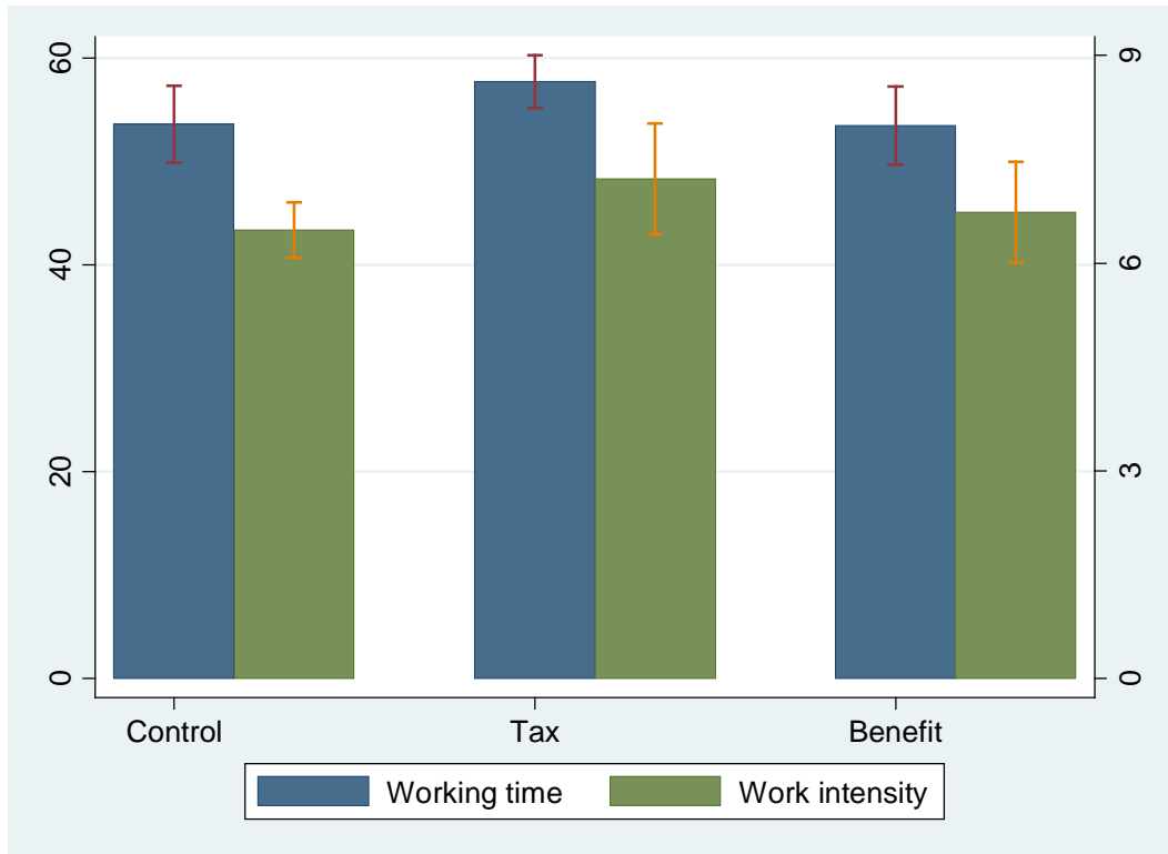
Figure 2: Mean working time and mean work intensity by treatment group
