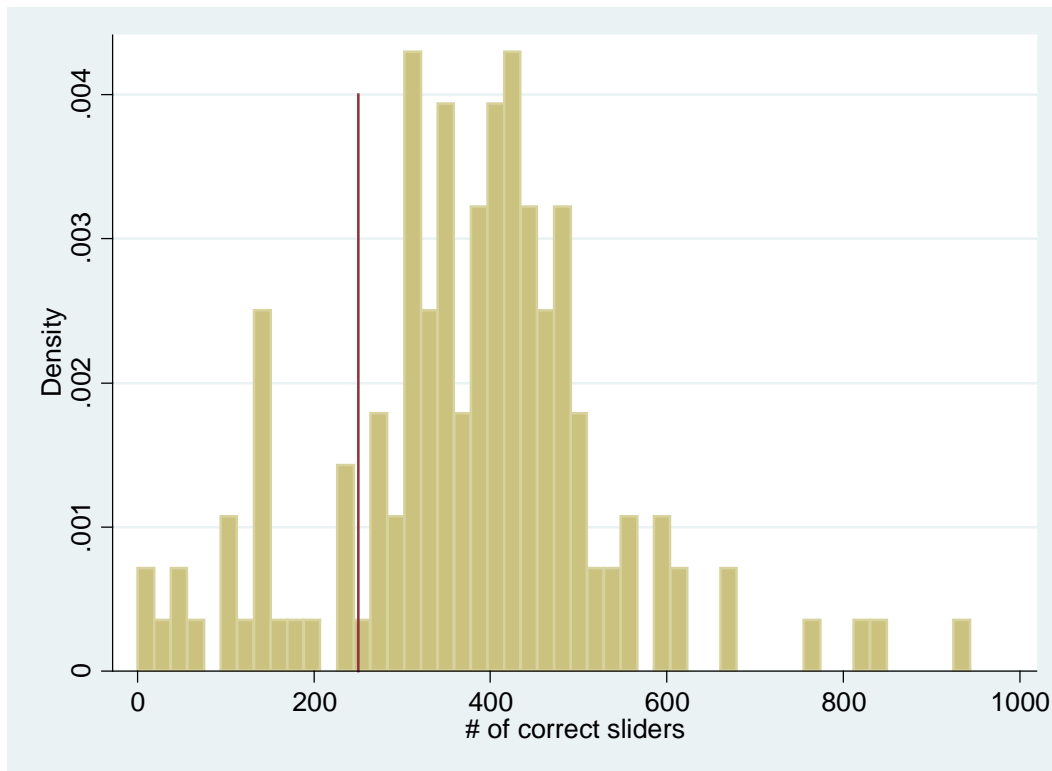
Figure 1: Distribution of number of correctly positioned sliders
