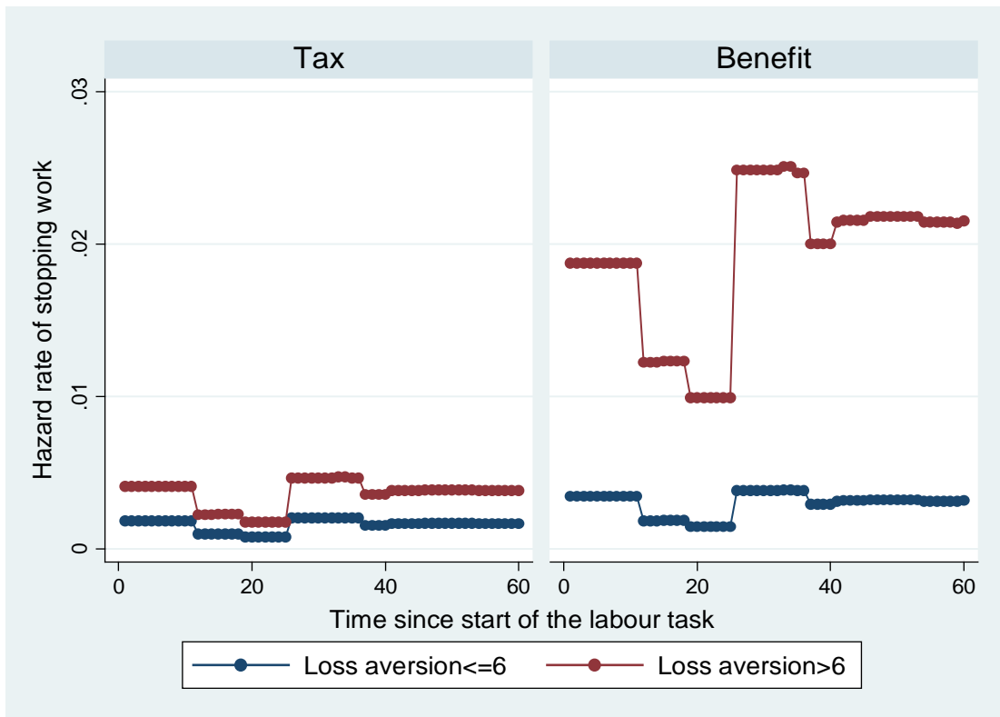
Figure 5: Predicted hazard rates of stopping work by treatment and loss aversion status
