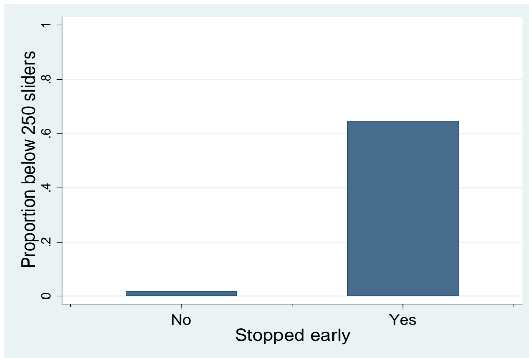
Figure 3: Proportion not reaching the 250 th slider by working time
