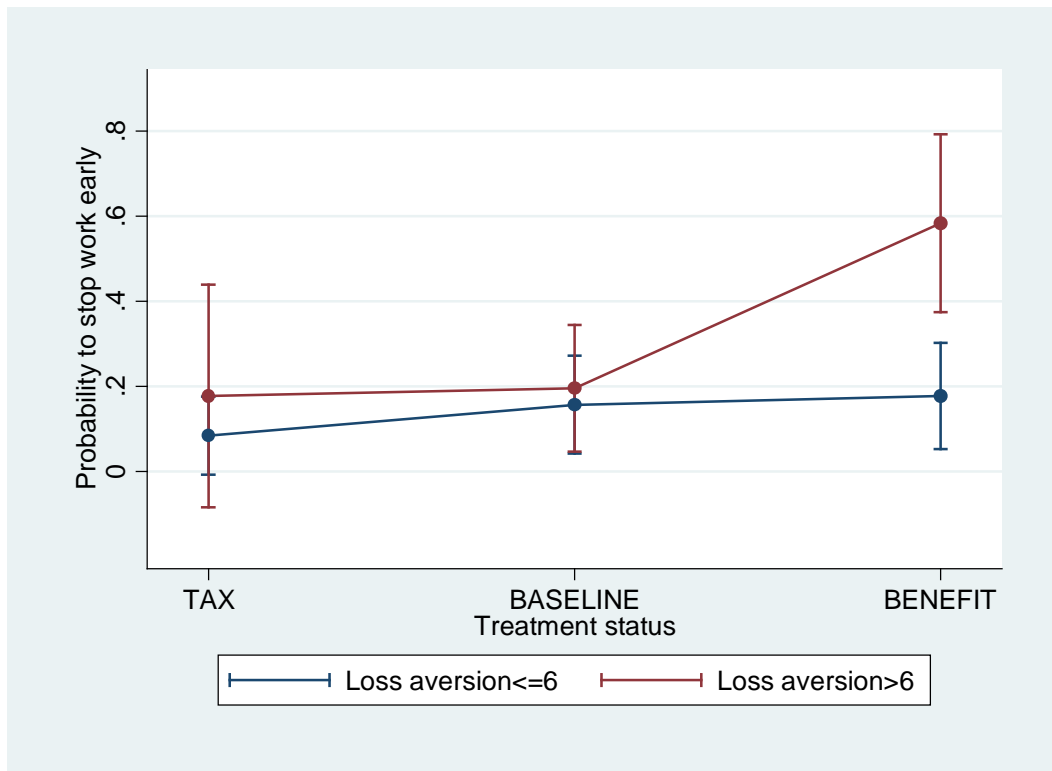
Figure 4: Probability of stopping early by treatment group and loss aversion score
