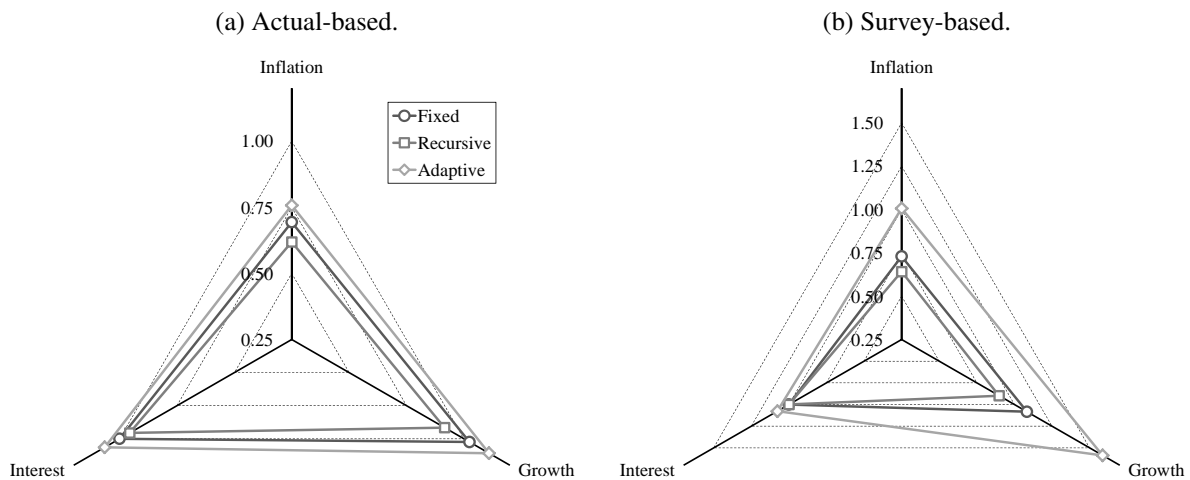
Figure 7: Averaged gain values using revised data relative to real-time calibrations.
