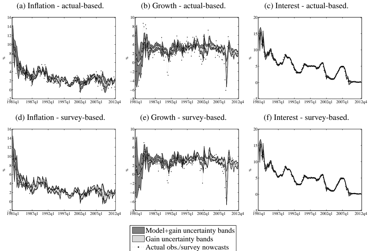
Figure 5: Evolution of nowcasts variability between models and calibrations.
