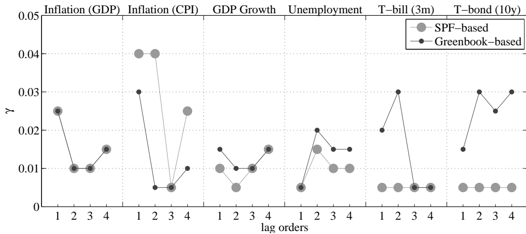
Figure 8: Policymakers fixed gain calibrations.
