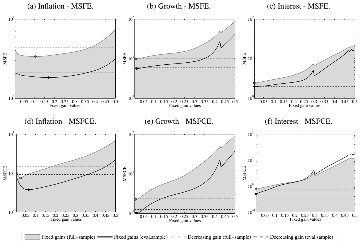
Figure 1: Forecasting performance curves.
