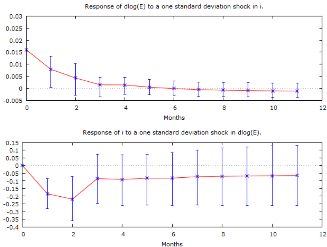
Figure A2.1. Impulse responses.
