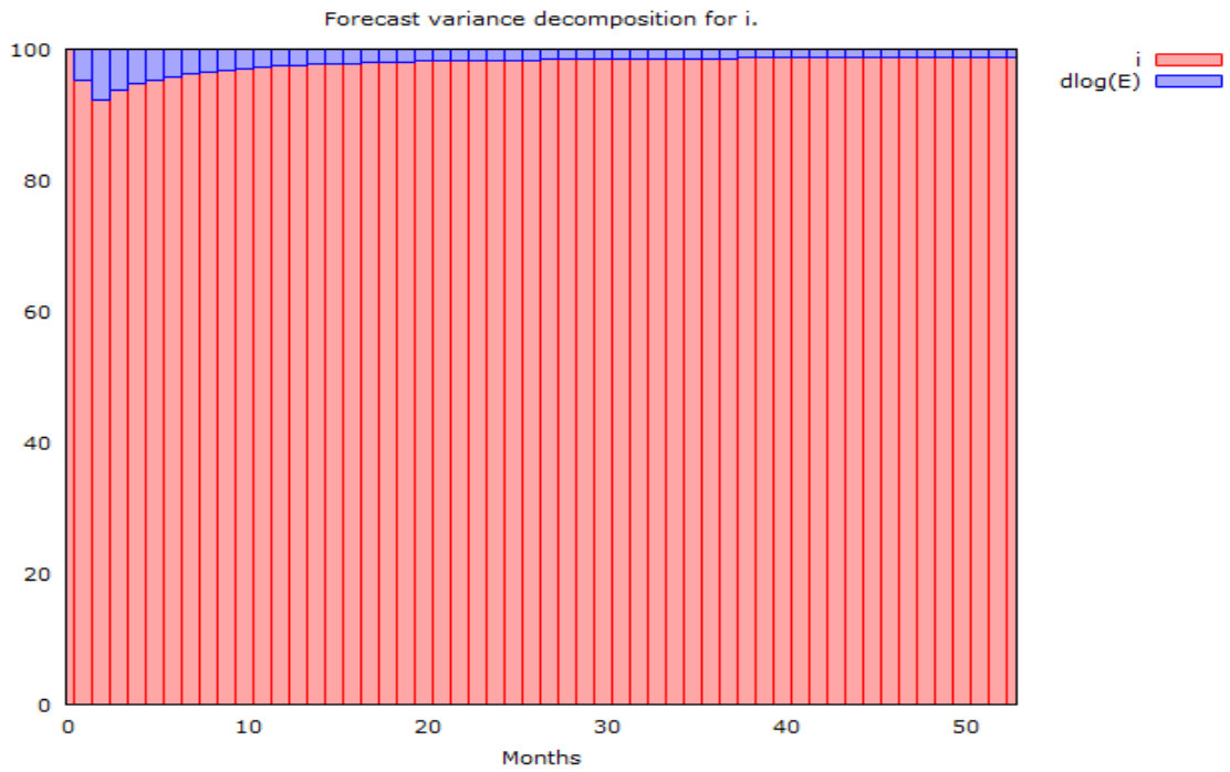
Figure A2.2. Variance decomposition for the policy interest rate.
