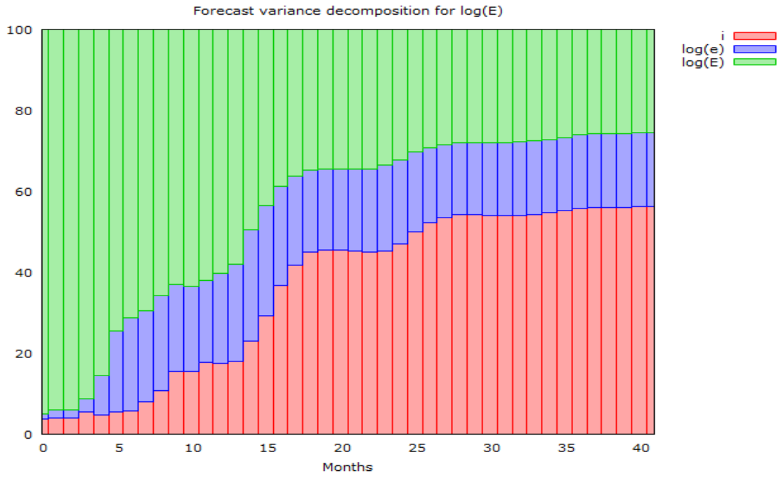
Figure A3.3. Variance decomposition for the onshore exchange rate.
