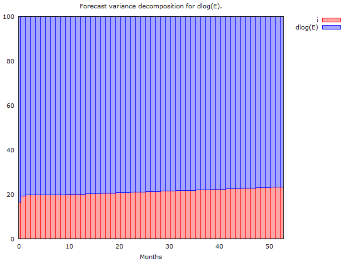
Figure A2.3. Variance decomposition for the exchange rate.
