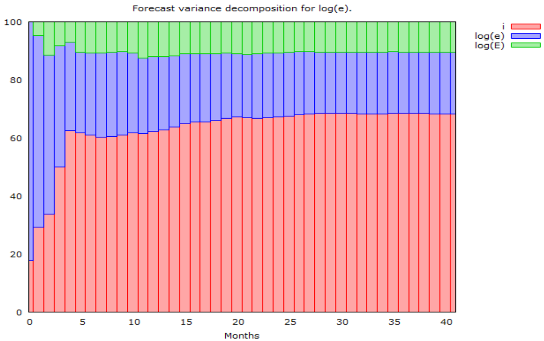
Figure A3.2. Variance decomposition for the offshore exchange rate.
