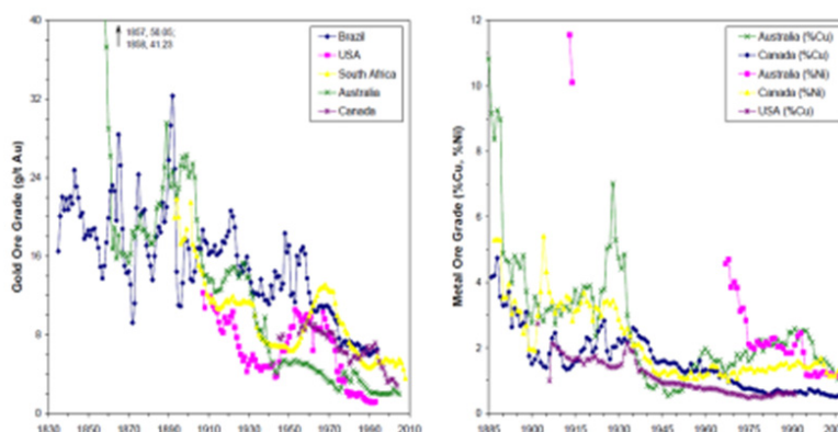
Figure 5: The decline of ore grades of gold, copper and nickel mines worldwide during the past century
