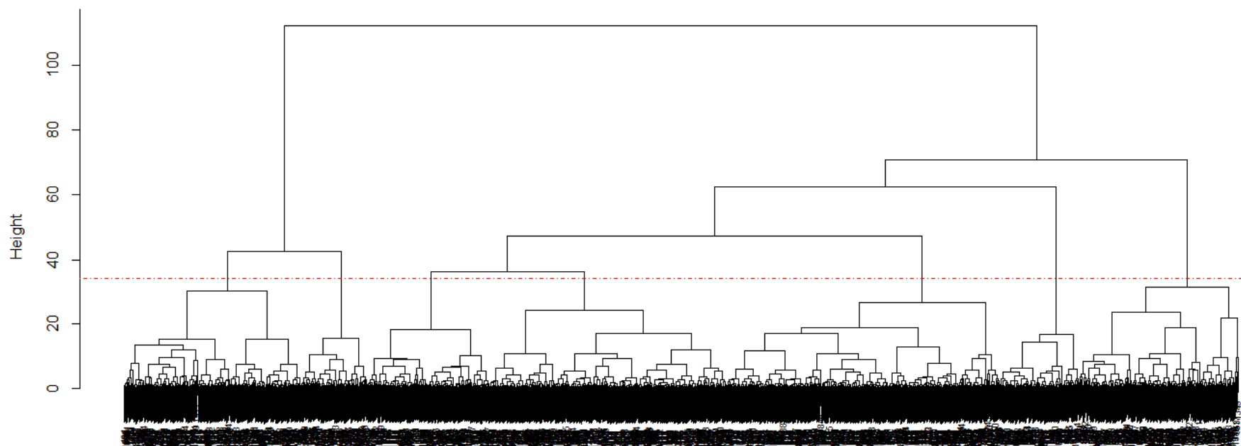
Figure 48 – Dendrogram
