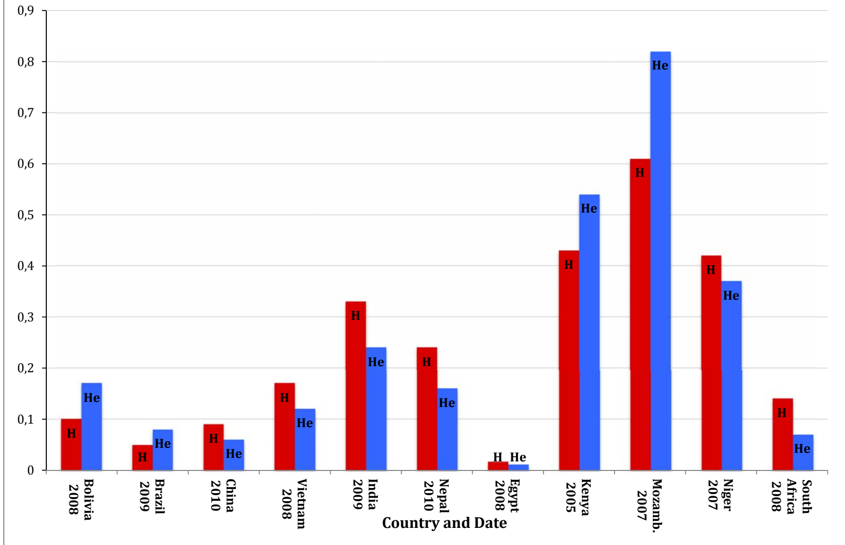
Figure 3: Comparison of Headcount Ratio and Person-Equivalent Head Count Ratio for Selected Countries
