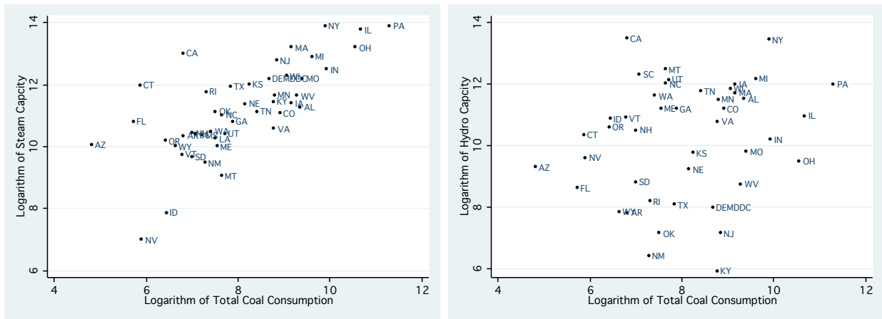
Figure 4: State-level Coal Consumption, Coal-Fired Capacity, and Hydroelectric Capacity
