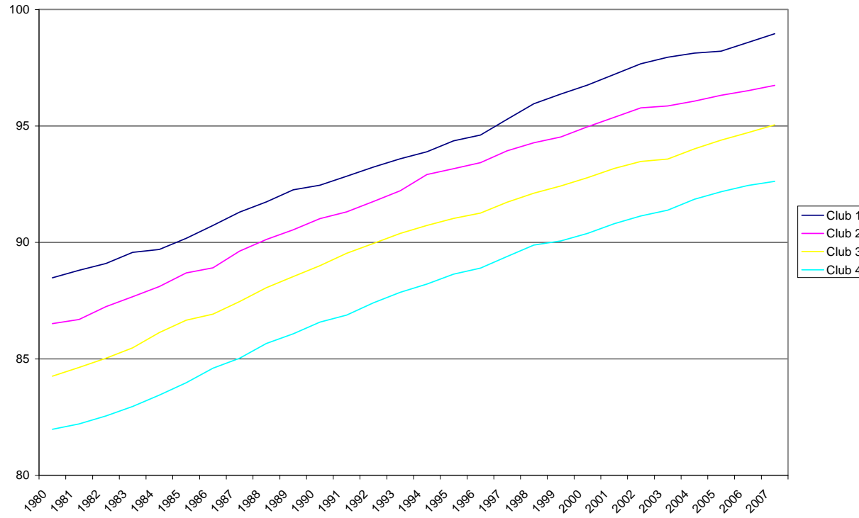
Fig 2. Club Indices
