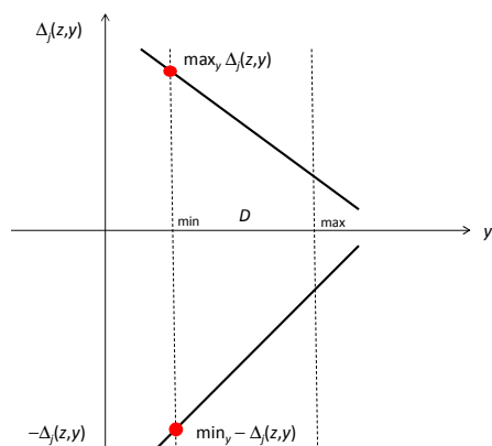
Figure 1. Cournot-Nash equilibrium (Theorem 1)
