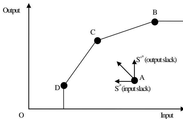
Figure 4 Illustration of the non-radial model in input/output space
