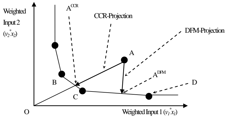
Figure 3 Degree of improvement of the DFM and the CCR projection in weighted input space
