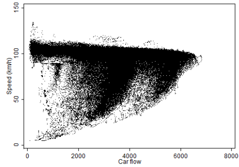
Figure A5 – Speed-flow relationship highway
