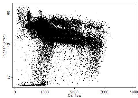
Figure A4 – Speed-flow relationship inner city roads
