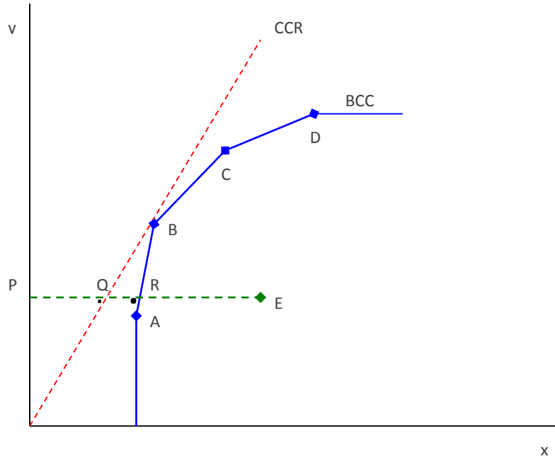
Figure 1: Frontiers of Efficiency CCR and BCC
