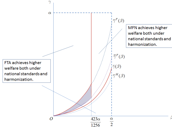
Figure 5: Comparison of the welfare effects of FTA between national standards and harmonization
