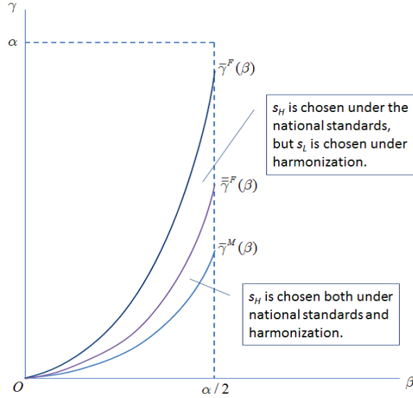
Figure 4: Harmonization of standards under the FTA
