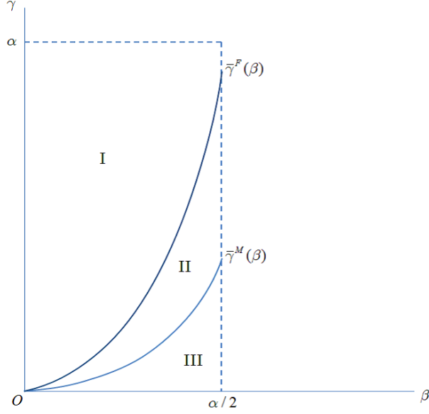
Figure 2: Comparison of optimal standards before and after an FTA
