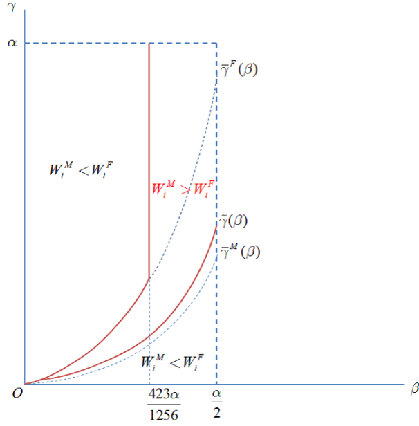
Figure 3: Comparison of the FTA members' welfare before and after an FTA
