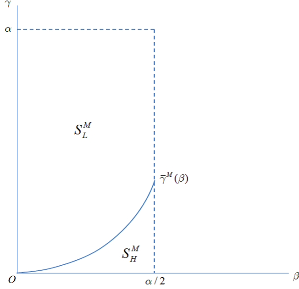
Figure 1: Optimal standards in the absence of FTAs
