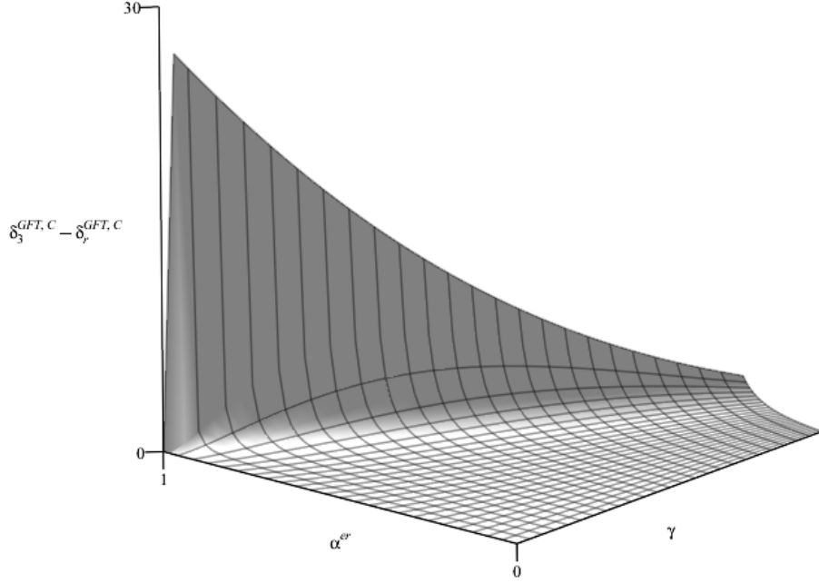
Figure A.1: \delta_3^{GFT,C} - \delta_r^{GFT,C}
