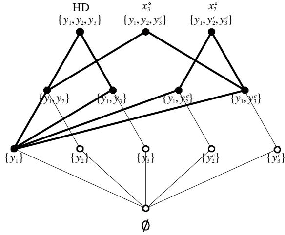
(a) Boolean sub-algebras of viable implication-sets
