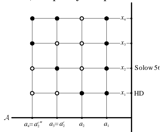
Figure 11: Boolean Algebras and Viable Models in Theory Space with \mathcal{A} = \{a_1, a_2, a_3 = a_2^c, a_4\}
