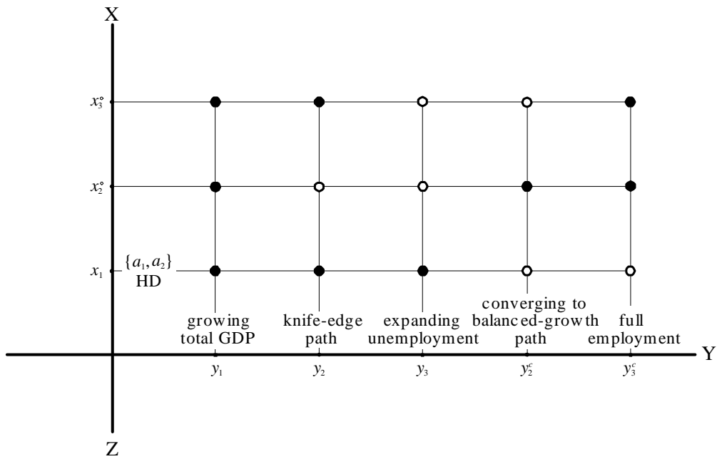
Figure 12: Boolean Algebras of Viable-Implication Sets and Potential Models in Science Space with \mathcal{Y} = \{y_1, y_2, y_3, y_2^c, y_3^c\}
