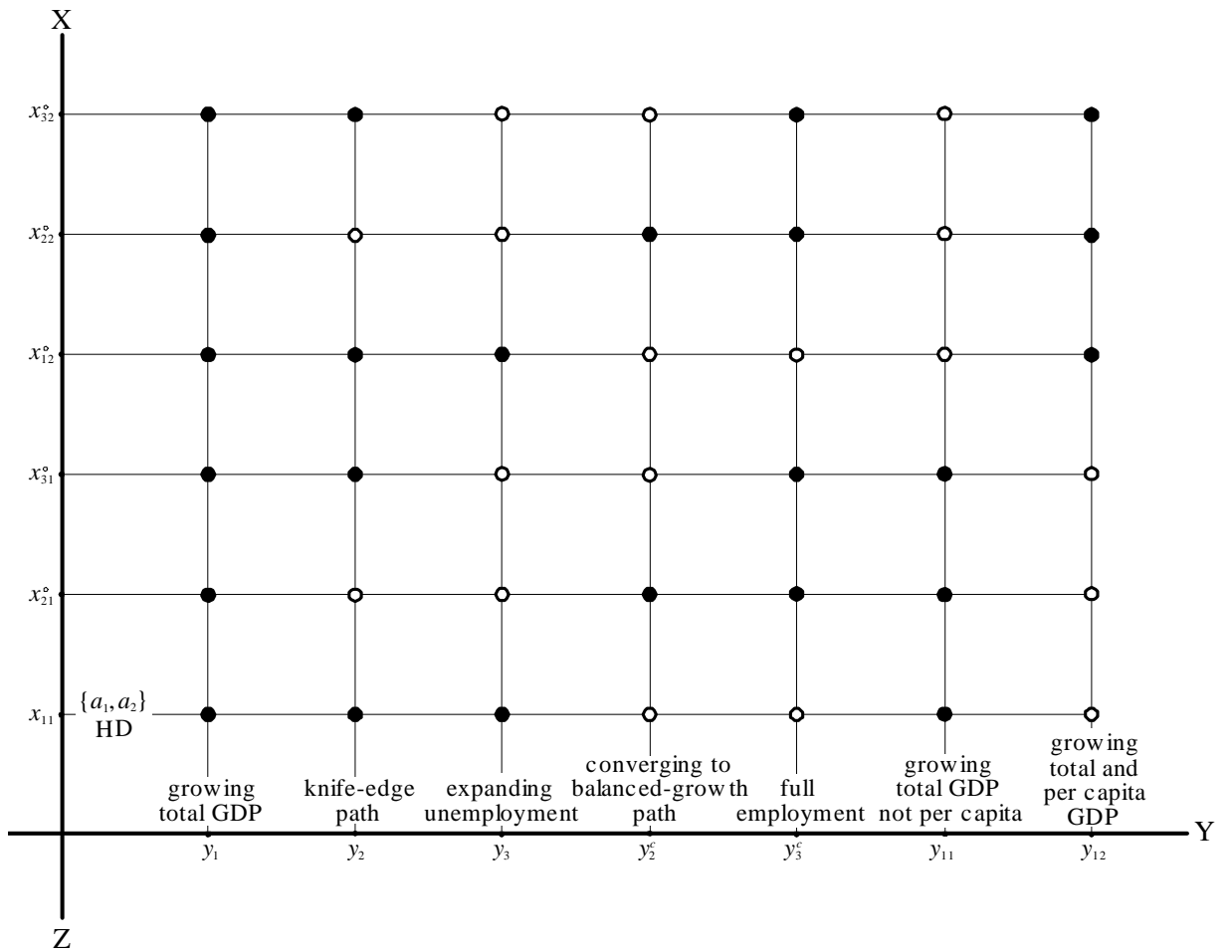
Figure 13: Viable implication-sets and potential models in Science space with \mathcal{Y} = \{y_1, y_2, y_3, y_2^c, y_3^c, y_{11}, y_{12}\}
