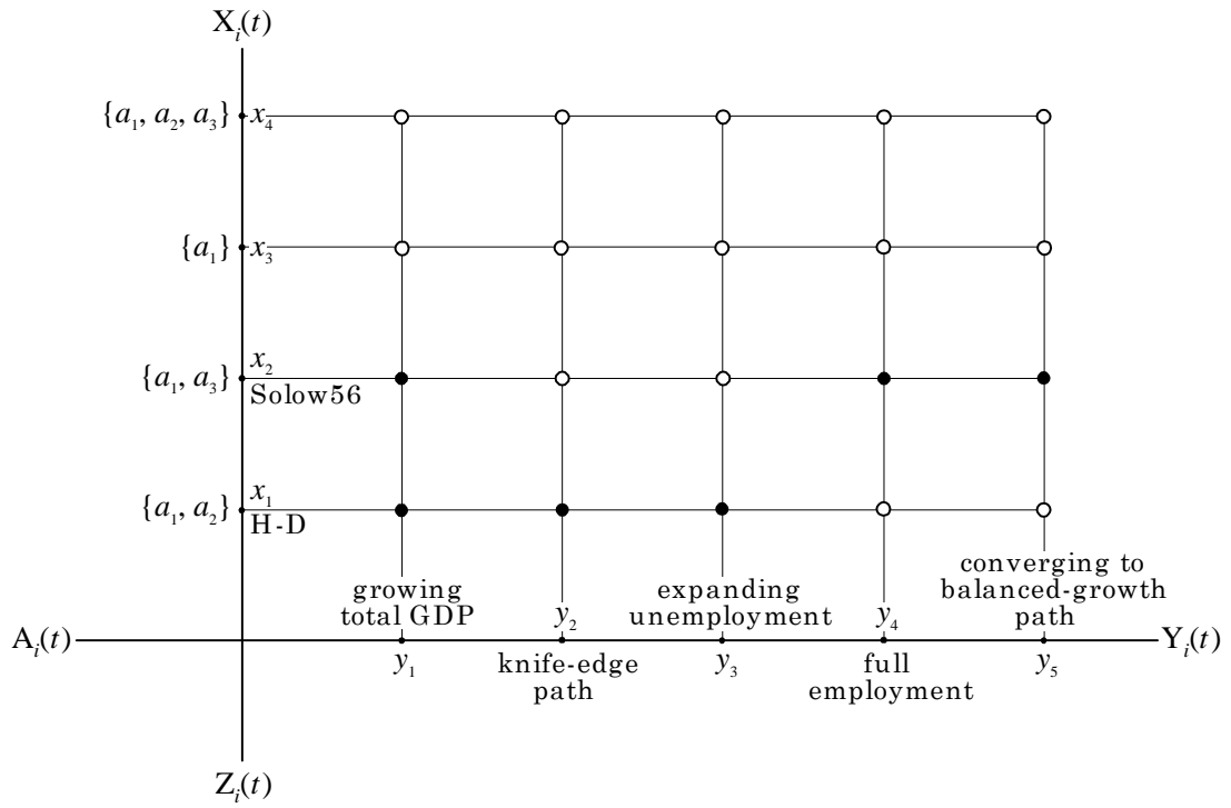
Figure 4: How to Work in Science Space
