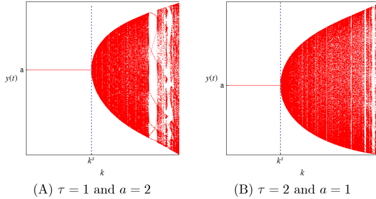
Figure 2. Bifurcation diagrams with different steps
