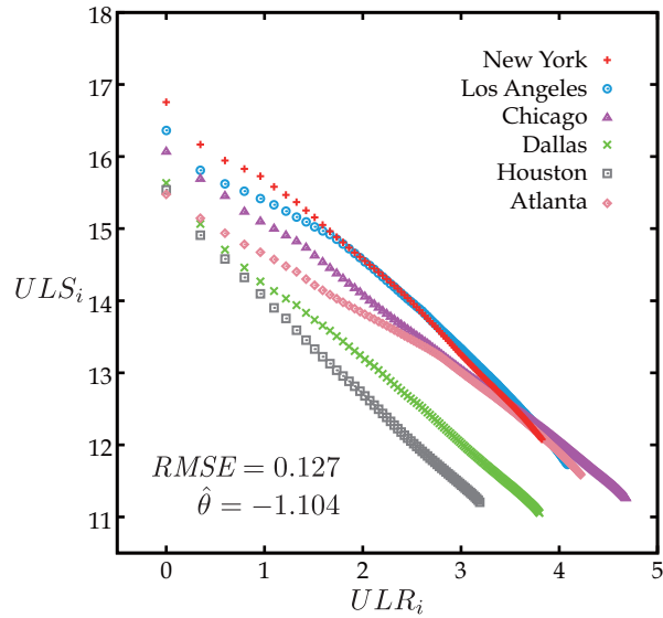
Figure 11: Upper-average distributions under (\lambda, K) = (0.05, 6)
