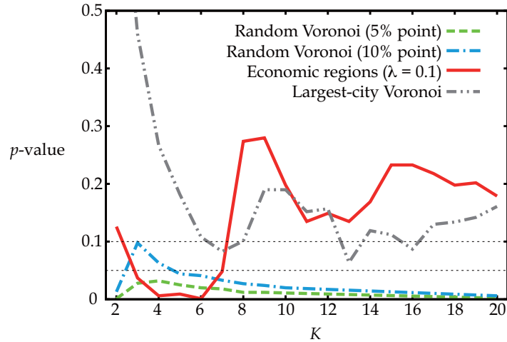
Figure 13: CPL Comparisons of Economic-Region and Voronoi Partitions
