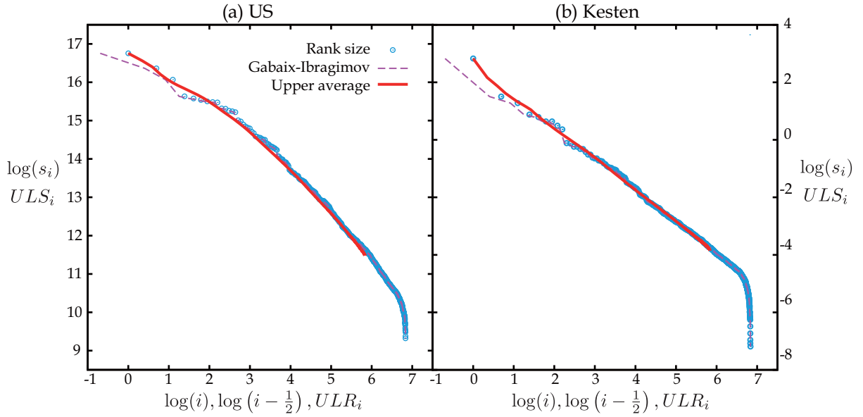
Figure 1: City size distribution from Kesten process
