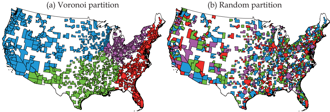
Figure 3: An example of Voronoi 4-partition
