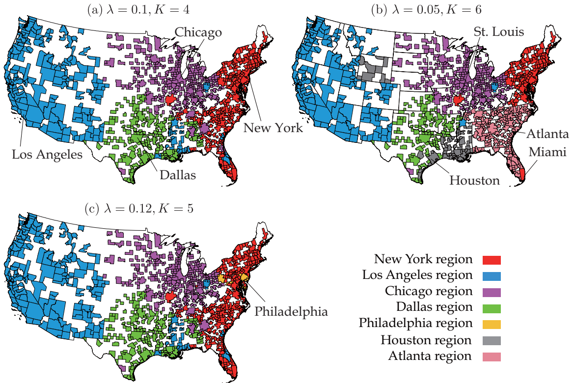
Figure 9: Economic regions for selected values of \lambda and K
