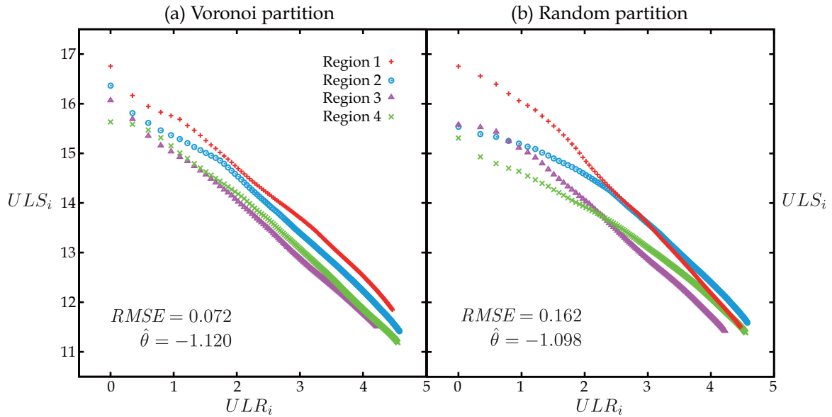
Figure 4: Upper-average distributions in Voronoi and random partitions
