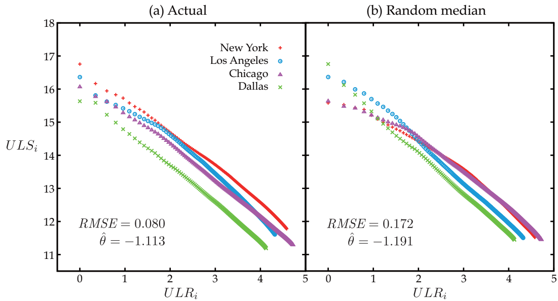
Figure 10: Upper-average distributions under (\lambda, K) = (0.1, 4)
