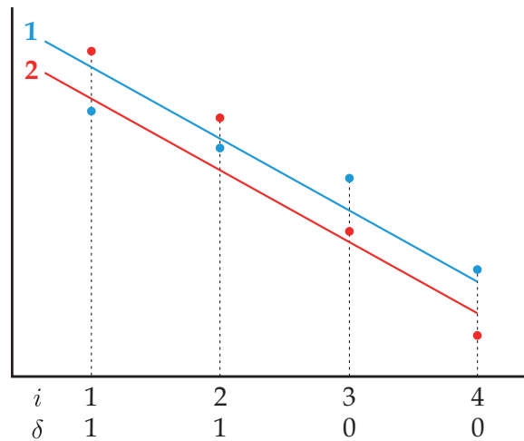
Figure 15: Categorical Regression Example
