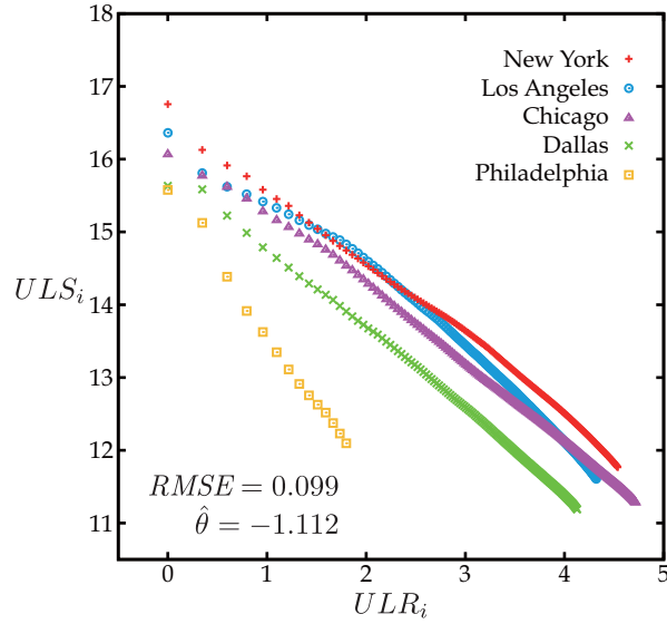
Figure 12: Upper-average distributions under (\lambda, K) = (0.12, 5)
