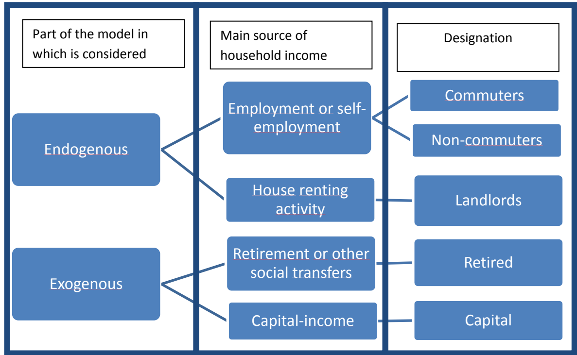
Figure 2: Different household's types considered in the MMRIO-Commuting Model
