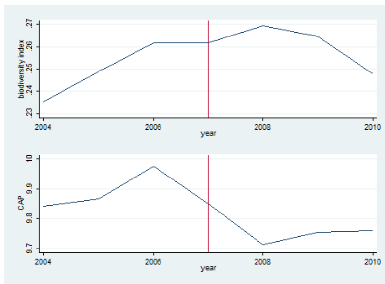
Figure 1: All sample means of biodiversity index (top) and CAP (bottom) over time
