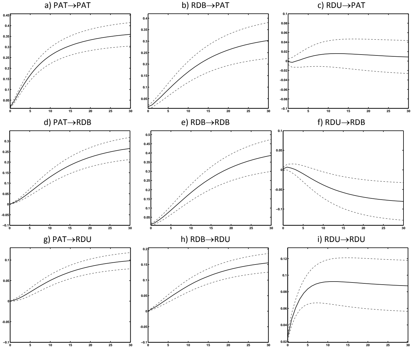
FIGURE 5. Space-time impulse response functions from the baseline model: spatial spillovers on 1 st order neighbors (1)
