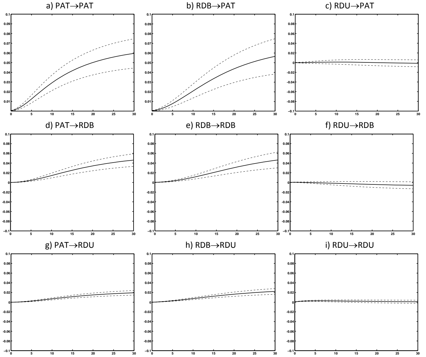
FIGURE 6. Space-time impulse response functions from the baseline model: spatial spillovers on 2 nd order neighbors (1)
