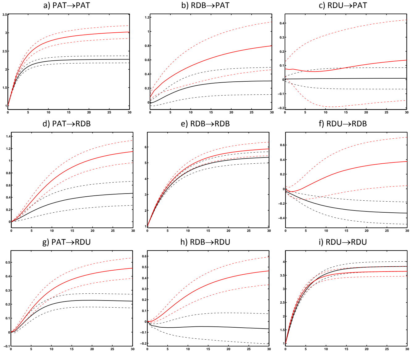
FIGURE 7. Space-time impulse response functions from the extended model: within region effects (1)
