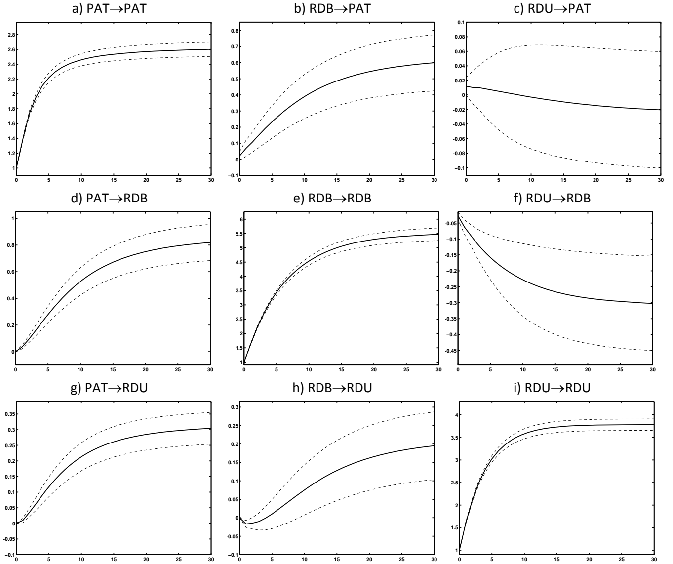
FIGURE 4. Space-time impulse response functions from the baseline model: within region effects (1)
